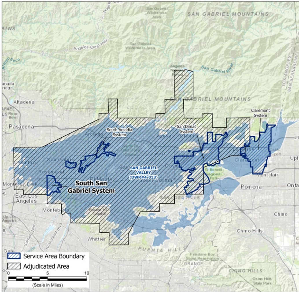
Figure 6-1 Groundwater Basins Underlying GSWC South Arcadia
