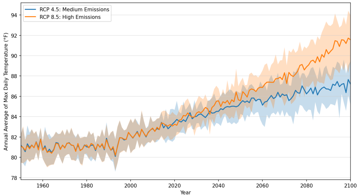
Figure 3-3 Observed and Forecasted Temperature for GSWC South Arcadia's Service Area
